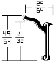
Outside Rubber Strip
