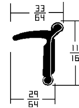
Outside Rubber Strip
