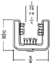
Flexible Window Channel
