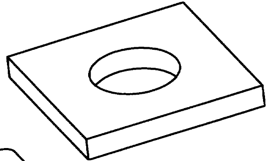
990413.....$5.00Ea 40-58 Buick Mount Pad 2" X 2" X 1/4" Thick 15/16" Hole
