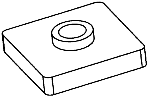
BM40A.....$5.50Ea 40 Buick Body Mount Pad 2" X 2" X 3/8" Thick
