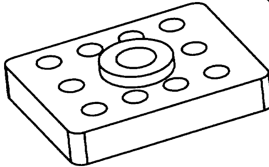
20013.....$6.50Ea 40 Buick & Others 2-1/4" X 1-3/4" 3/8" Thick Collar 3/4" X 1/8" Thick 3/8" Hole
