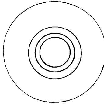
MTHLG1.....$17.000Ea Mack Truck A-20 Headlight Grommet, 2-1/2" Od, 7/8" Hole, 1/2" Overall Thickness
