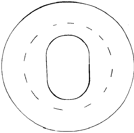
MTPG1.....$18.00Ea Mack Truck Pedal Grommet, 4-1/2" Od, 1/8" Groove, 1-1/2" X 2-1/8" Oval Hole
