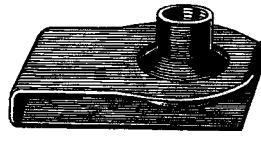
10052.....95Ea 5/16-18 Screw Panel Range .025"-.150", Ctr Of Hole To Edge 7/8"
