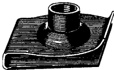
10053.....60Ea 5/16-18 Screw Panel Range .025"-.150", Ctr Of Hole To Edge 9/16"
