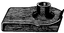
8814.....95Ea 5/16-18 Screw Panel Range .025"-.150", Ctr Of Hole To Edge 27/32"
