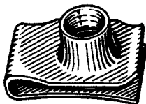
10227.....$1.25Ea 5/16-18 Screw Panel Range .040"-.080", Ctr Of Hole To Edge 5/8"
