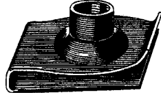
12265.....60Ea 5/16-18 Screw Panel Range .040"-.125", Ctr Of Hole To Edge 9/16"
