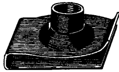
10830.....60Ea 5/16-18 Screw Panel Range .025"-.150". Ctr Of Hole To Edge 5/8"
