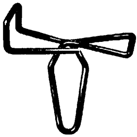
2166.....$1.25Ea Body Side Shield Mld Fastener Buick 41-42 Models 40, 60 & 90; Front Fender Lower Mld Fastener Buick 41-42
